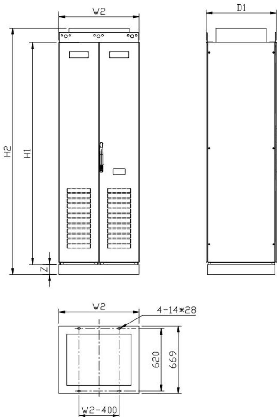
整流回馈 HF680N02C-250-4、HF680N02C-315-4、HF680N02C-400-4、HF680N02C-450-4 成柜外形示意图
